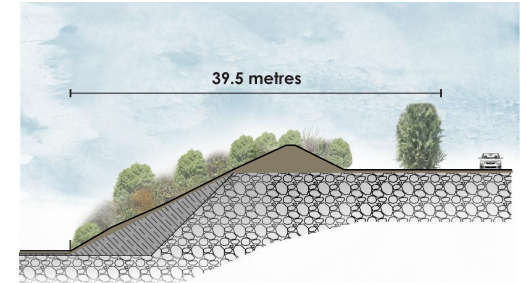
Section A-A: Aylesbury Road rehabilitation
