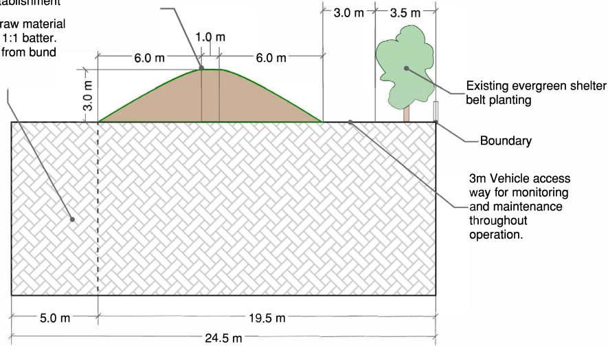
Fig A: Long-Term Edge Treatment
