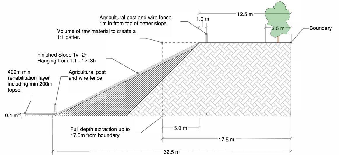
Fig B: Edge Treatment During Active Extraction
