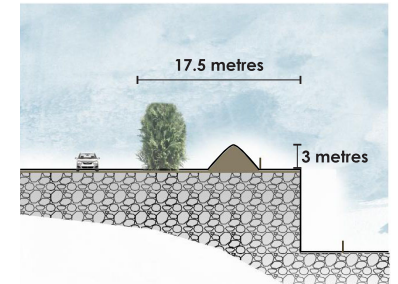
Section B-B: Grange Road excavation
