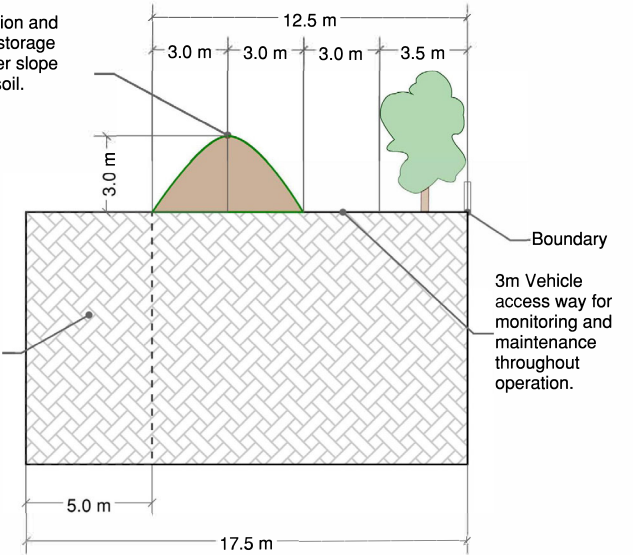
Fig B: Edge Treatment During Active Extraction
