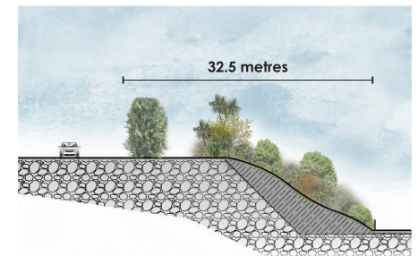
Section B-B: Grange Road rehabilitation
