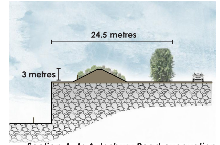
Section A-A: Aylesbury Road excavation
